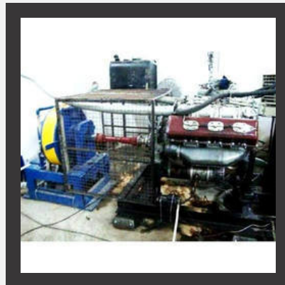
Engine Dyno Setup
